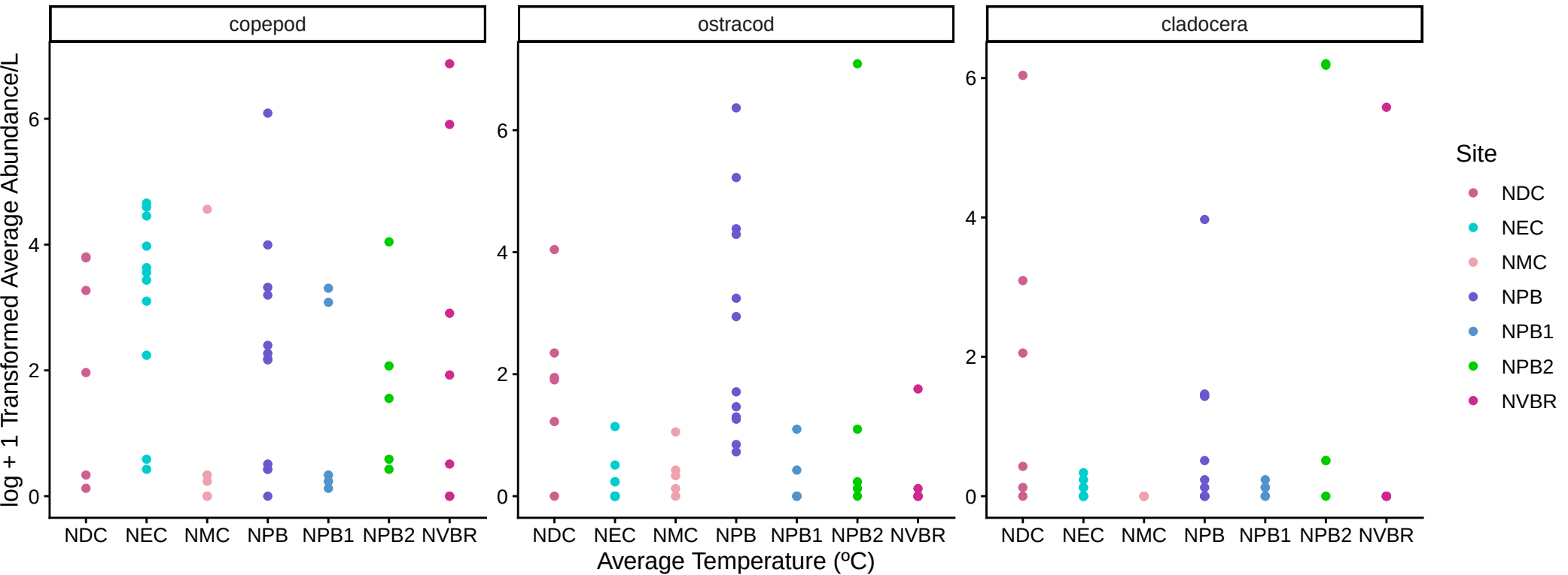
Average Abundance and Average Water Temperature for Three Dominant Taxa by Site
